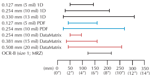
Bar Code Minimum Element
